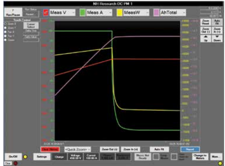
Figure 2 - Chart Recorder
