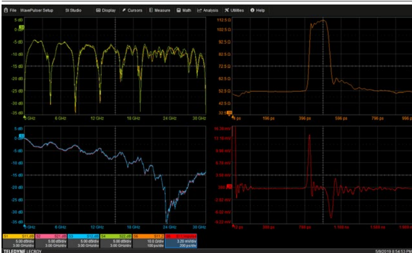
WavePulser 40iX step and impulse response combined with S-parameters enables determination of the type of impairment.
