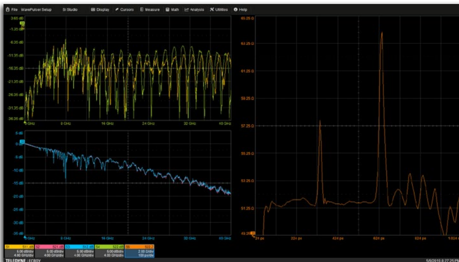
The impedance profile shows that one of the two through vias is defective.
