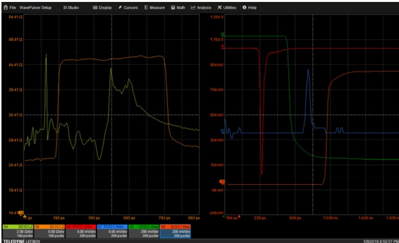
Impedance profile displays both common and differential modes.
