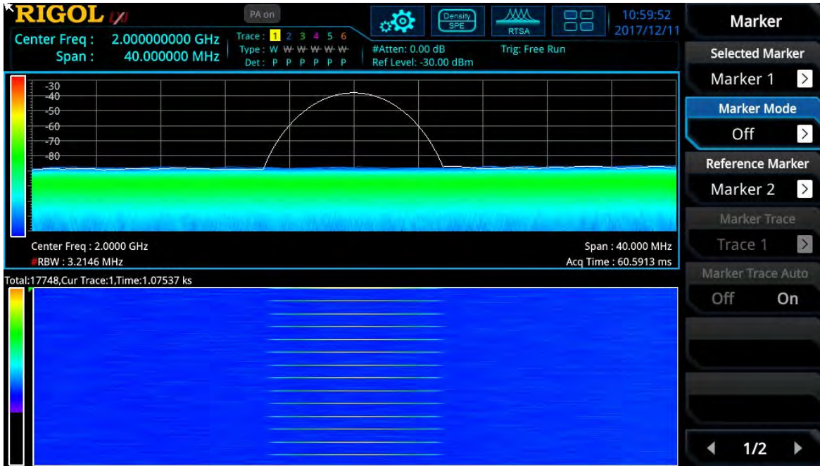
Figure 7: Measurement of a pulse of 7.45 \mu sec. (period: 1 sec.) with amplitude of -35 dBm. Each pulse is captured with correct amplitude.
